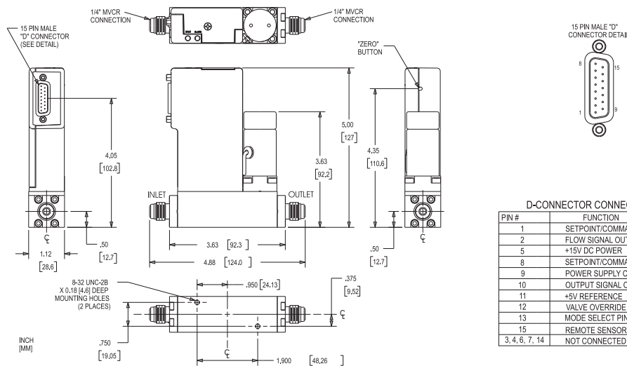
SLA7840D Digital I/O DeviceNet Controller with 1/4" VCR Connections
