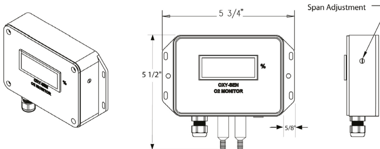
Outline dimensions
